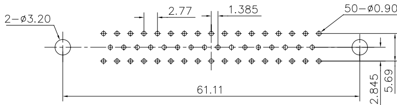
RECOMMENDED P.C.B LAYOUT (TOLERANCE +/-0.03)
