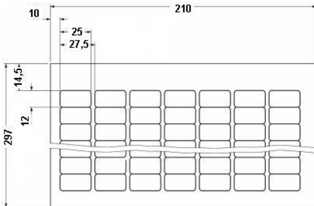
Dimensional drawing
