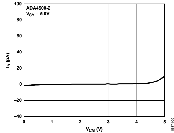
Figure 15. Input Bias Current ( I b ) vs. Common-Mode Voltage ( V CM ), V SY = 5.0 V
