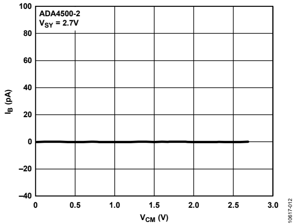
Figure 12. Input Bias Current ( I b ) vs. Common-Mode Voltage ( V CM ), V SY = 2.7 V
