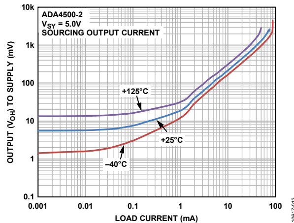
Figure 16. Output Voltage ( V OH ) to Supply Rail vs. Load Current, V SY = 5.0 V
