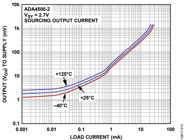
Figure 13. Output Voltage ( V OH ) to Supply Rail vs. Load Current, V SY = 2.7 V
