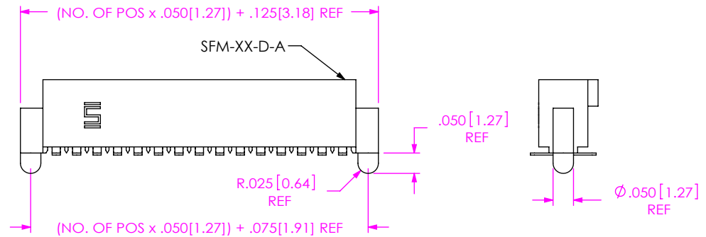
FIG 4 -A: ALIGNMENT PIN (SAME AS FIG 2, DIFFERENT AS SHOWN)
