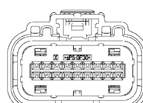
Keying Option “B”
