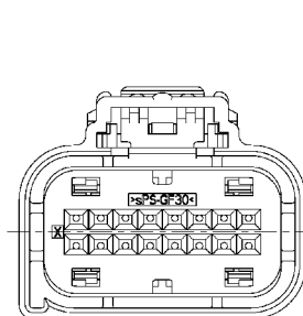
Keying Option "D" (Housing Color : Green)
