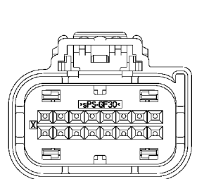
Keying Option "A" (Housing Color: Black)
