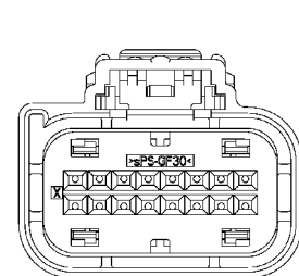
Keying Option "B" (Housing Color: Grey)
