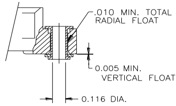
VARIATION 03 .116 ±.003 I.D. FLOATING EYELET
