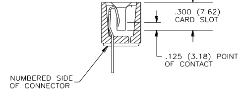
SINGLE ROW CONTACTS READ ONE SIDE OF DAUGHTER BOARD
