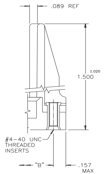
MOUNTING OPTION CODE #78
