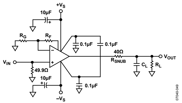
Figure 54. Typical Capacitive Load Configuration (SOIC)
