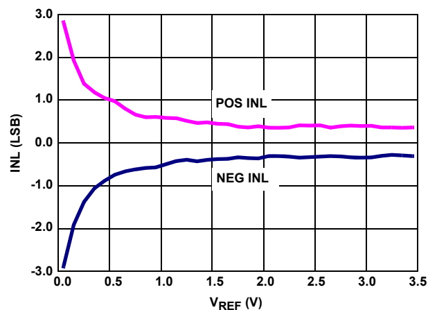
FIGURE 12. CHANGE IN INL vs V_{REF} FOR V_{DD} = 5V
