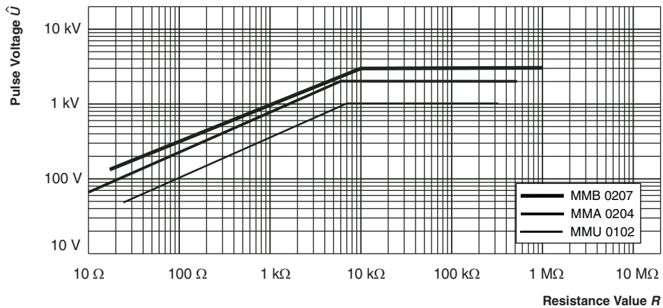
Pulse load rating in accordance with IEC 60115-1, 4.27; 1.2 μs/50 μs; 5 pulses at 12 s intervals; for permissible resistance change \pm (0.5\% R + 0.05 \Omega)
