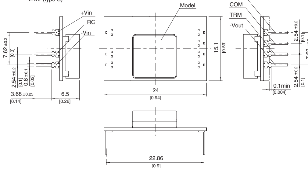
2.DIP(type C)
