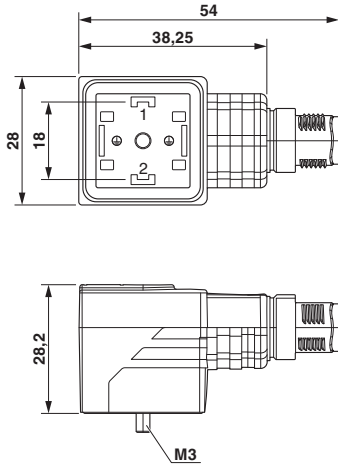
Dimensional drawing
