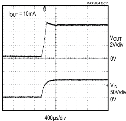
STARTUP RESPONSE
