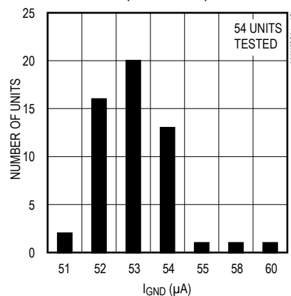
GROUND CURRENT DISTRIBUTION (T A = +125°C)
