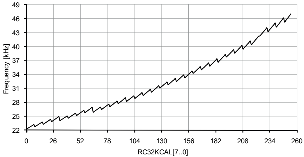
Figure 37-70. 32.768kHz internal oscillator frequency vs. calibration value.
