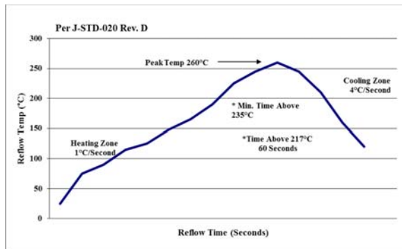
Figure 23. Recommended linear reflow profile using Sn/Ag/Cu solder.
