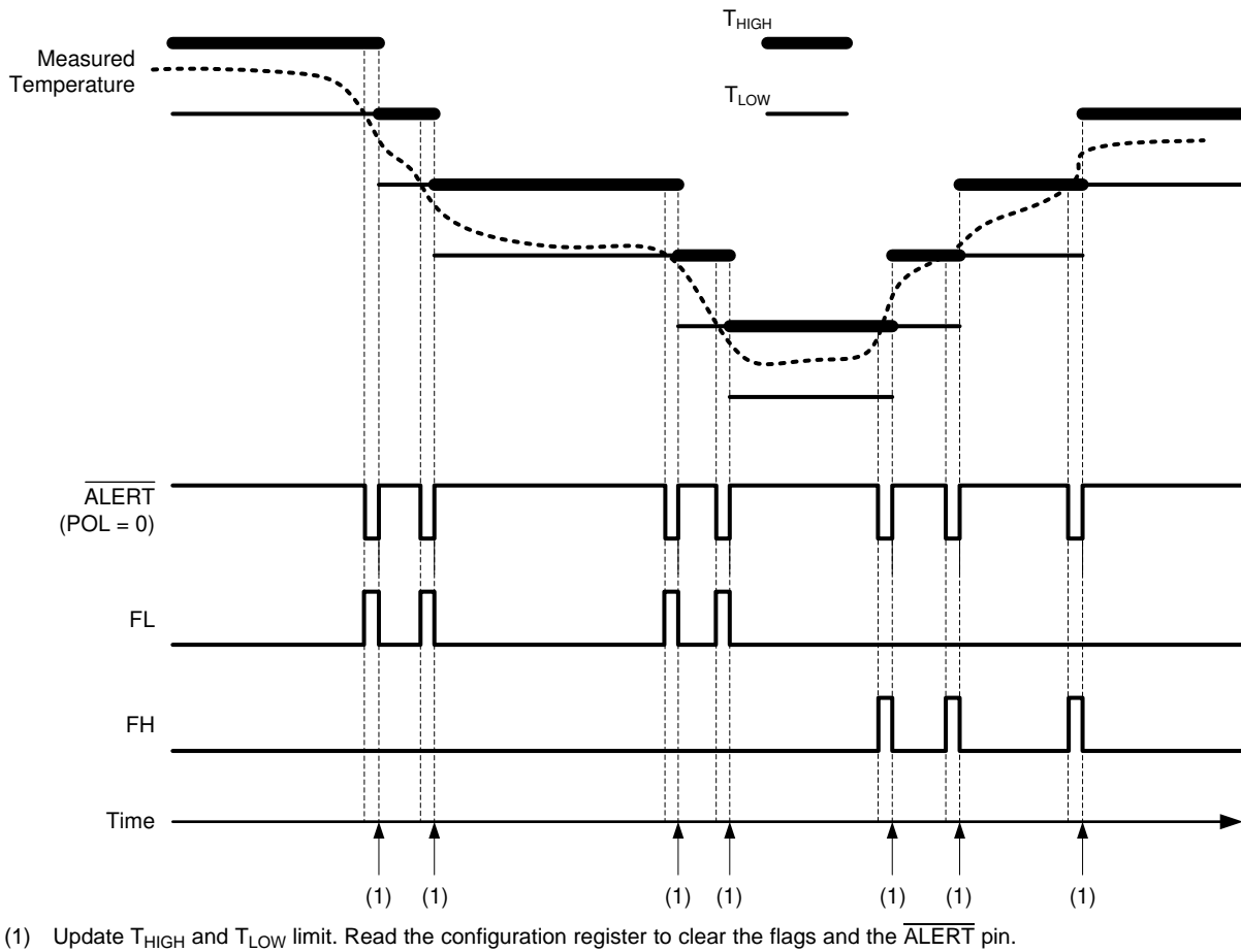
Figure 13. Interrupt Mode
