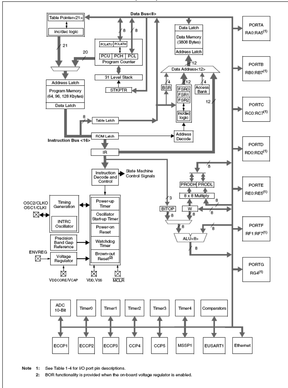
FIGURE 1-1: PIC18F66J60/66J65/67J60 (64-PIN) BLOCK DIAGRAM
