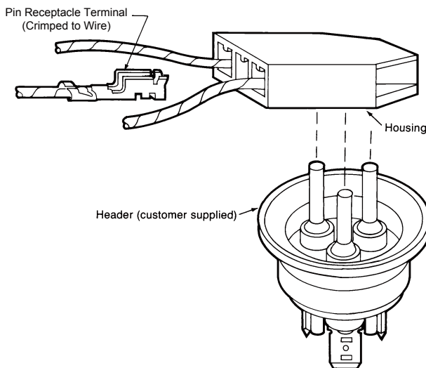
Typical Assembly
