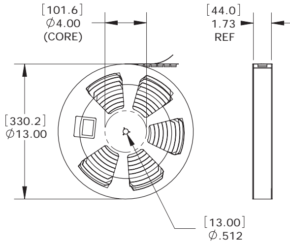
REEL INFORMATION (250 UNITS PER REEL)
