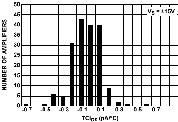
FIGURE 19. TCI OS- vs NUMBER OF AMPLIFIERS, V S = ±15V
