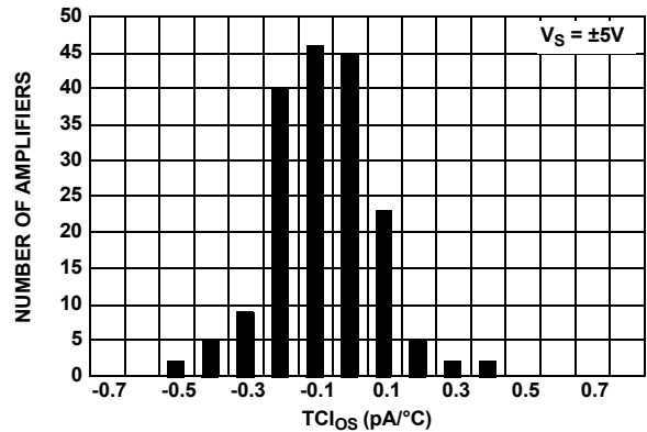
FIGURE 20. TCI OS- vs NUMBER OF AMPLIFIERS, V S = ±5V
