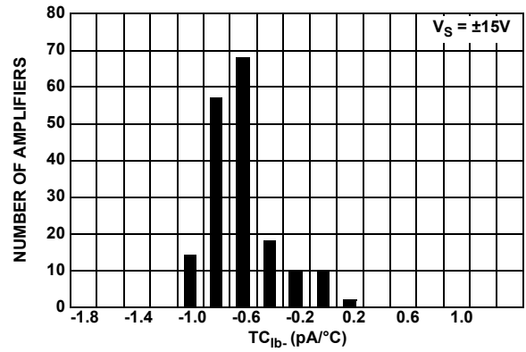
FIGURE 16. TC IBM vs NUMBER OF AMPLIFIERS, V S = ±15V
