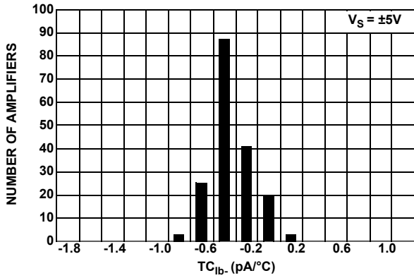
FIGURE 15. TC IBM vs NUMBER OF AMPLIFIERS, V S = ±5V
