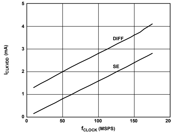
Figure 84. I_{CLKVDD} vs. f_{CLOCK} at CLKVDD = 3.3 V
