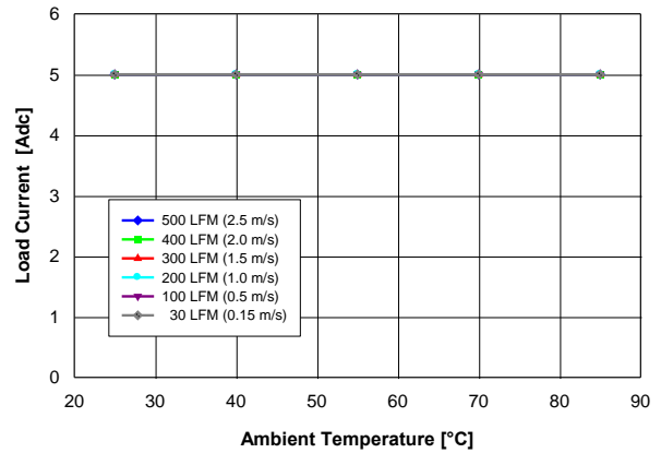
Fig. 1.5V.2: Available load current vs. ambient temperature and airflow rates for V_{out} = 1.5V converter mounted horizontally with V_{in} = 5 V , air flowing from pin 5 to pin 1 and maximum MOSFET temperature \leq 120^\circ C .
