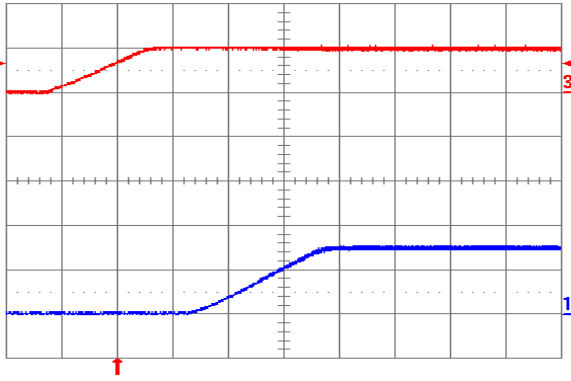
Fig. 1.5V.5: Turn-on transient for V_{out} = 1.5\text{ V} with application of V_{in} at full rated load current (resistive) and 47\ \mu\text{F} external capacitance at V_{in} = 5\text{ V} . Top trace: V_{in} ( 5\text{ V/div.} ); Bottom trace: output voltage ( 1\text{ V/div.} ); Time scale: 2\text{ ms/div.}
