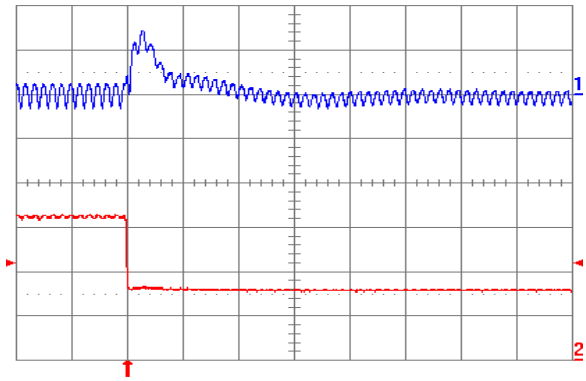
Fig. 3.3V.8: Output voltage response for V_{out} = 3.3\text{ V} to negative load current step change from 5\text{ A} to 2.5\text{ A} with slew rate of -5\text{ A}/\mu\text{s} at V_{in} = 5\text{ V} . Top trace: output voltage ( 100\text{ mV}/\text{div.} ); Bottom trace: load current ( 2\text{ A}/\text{div.} ). C_o = 47\text{ }\mu\text{F} ceramic + 1\text{ }\mu\text{F} ceramic. Time scale: 20\text{ }\mu\text{s}/\text{div.}
