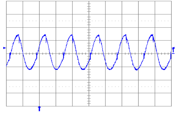
Fig. 1.5V.6: Output voltage ripple ( 20\text{ mV/div.} ) at full rated load current into a resistive load with external capacitance 10\ \mu\text{F} ceramic + 1\ \mu\text{F} ceramic and V_{in} = 5\text{ V} for V_{out} = 1.5\text{ V} . Time scale: 2\ \mu\text{s/div.}
