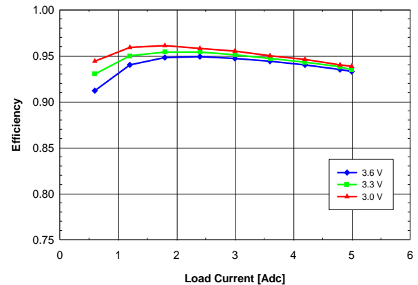
Fig. 2.5V.4: Efficiency vs. load current and input voltage for V_{out} = 2.5\text{ V} converter mounted vertically with air flowing from pin 5 to pin 1 at a rate of 200\text{ LFM} ( 1\text{ m/s} ) and T_a = 25\text{ }^\circ\text{C} .
