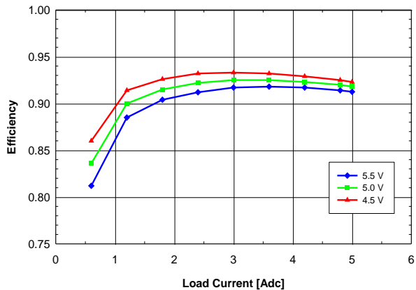
Fig. 2.5V.3: Efficiency vs. load current and input voltage for V_{out} = 2.5\text{ V} converter mounted vertically with air flowing from pin 5 to pin 1 at a rate of 200\text{ LFM} ( 1\text{ m/s} ) and T_a = 25\text{ }^\circ\text{C} .
