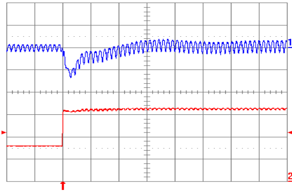
Fig. 3.3V.7: Output voltage response for V_{out} = 3.3\text{ V} to positive load current step change from 2.5\text{ A} to 5\text{ A} with slew rate of 5\text{ A}/\mu\text{s} at V_{in} = 5\text{ V} . Top trace: output voltage ( 100\text{ mV}/\text{div.} ); Bottom trace: load current ( 2\text{ A}/\text{div.} ). C_o = 47\text{ }\mu\text{F} ceramic + 1\text{ }\mu\text{F} ceramic. Time scale: 20\text{ }\mu\text{s}/\text{div.}
