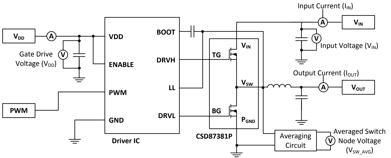
Figure 27. Typical Application
