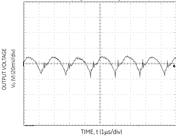
Figure 9. Typical output ripple and noise (C o =22µF ceramic, V IN = 12V, I o = I o,max ).
