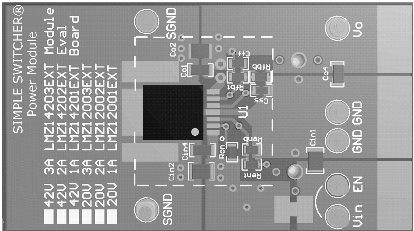
Figure 43. Bottom View of Board
