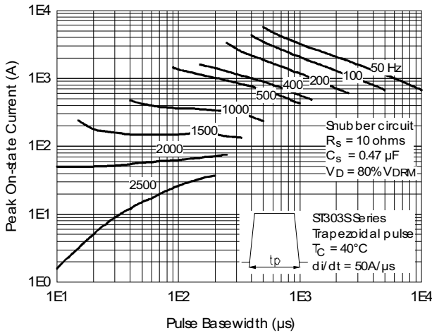
Fig. 12 - Frequency Characteristics
