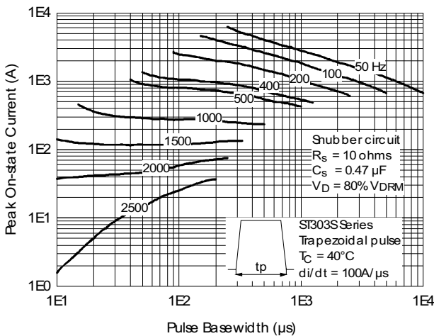
Fig. 13 - Frequency Characteristics
