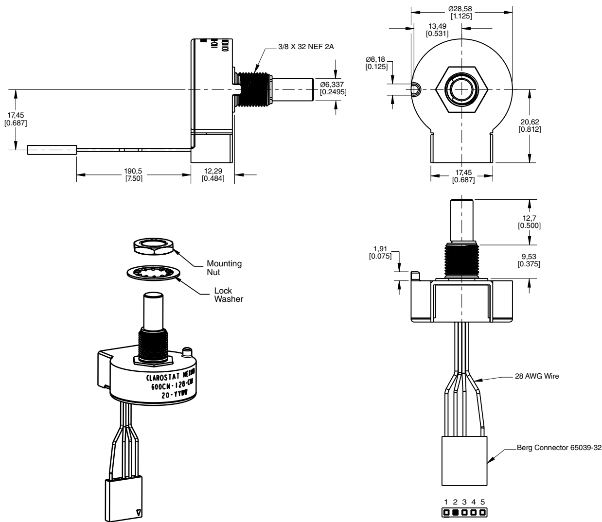
Figure 2. Mounting Hardware
