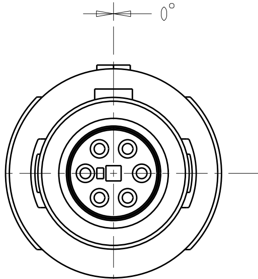
0° KEYING SCALE 4:1
