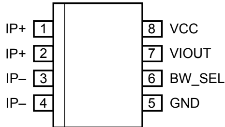
Pinout Diagram
