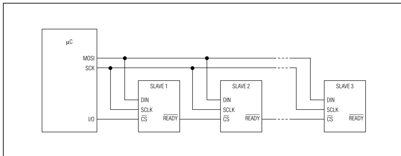
Figure 5. Daisy-Chain Configuration
