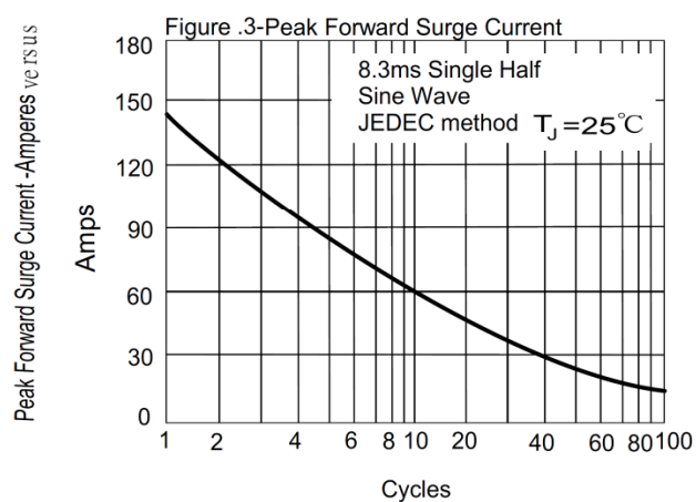
Number Of Cycles At 60Hz - Cycles
