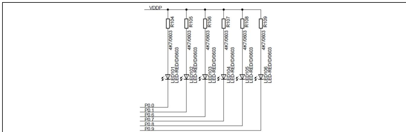
Figure 4 LEDs circuit
