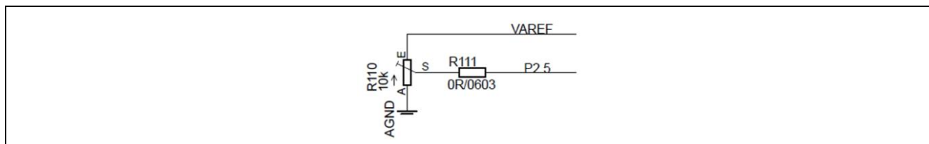
Figure 5 Potentiometer Circuit
