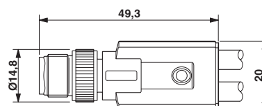
Dimensional drawing
