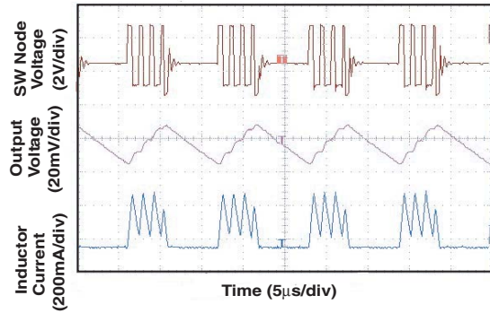
Figure 10. Power-Save Mode
