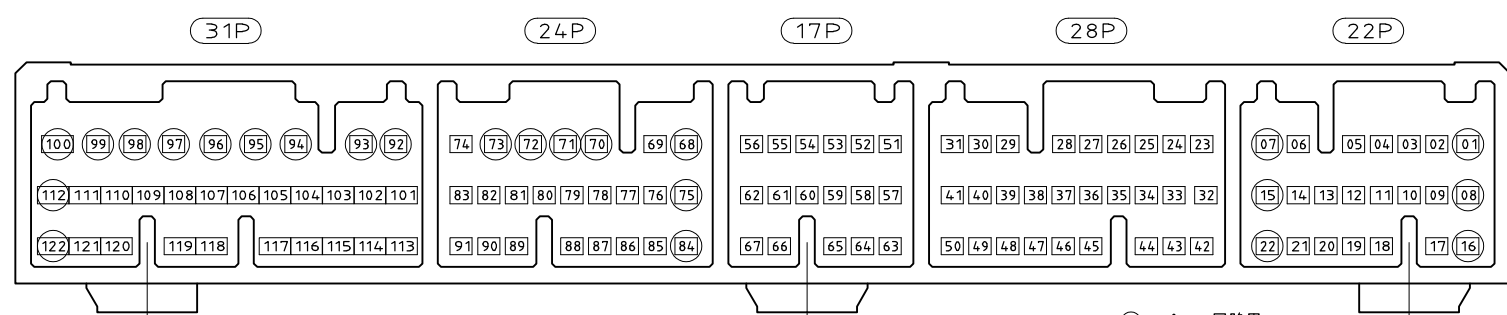
FIG 1 CIRCUIT NUMBERS (FOR POWER CIRCUIT)
