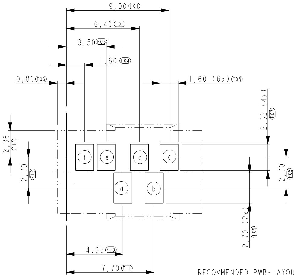
RECOMMENDED PWB-LAYOUT
