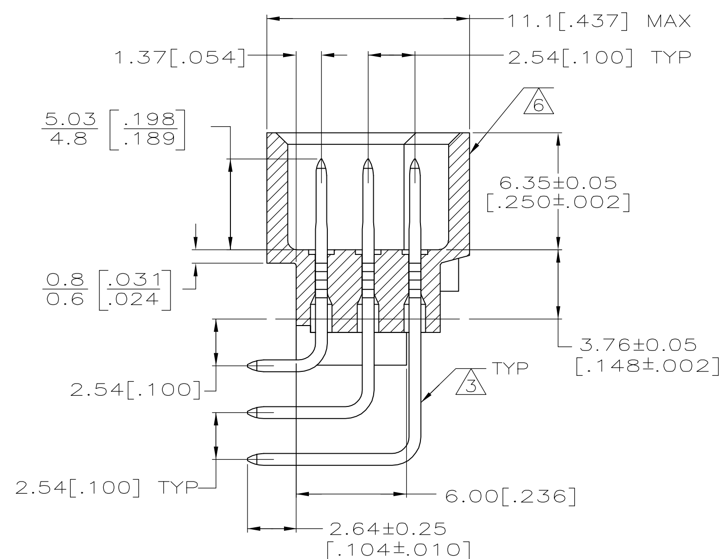
SECTION Z-Z
