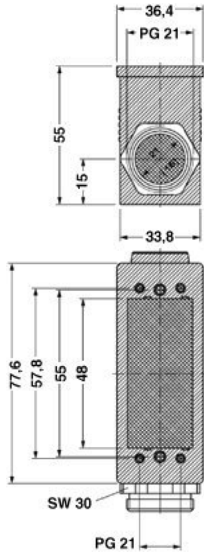
Dimensional drawing
