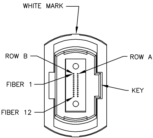
VIEW Z-Z NOT TO SCALE
