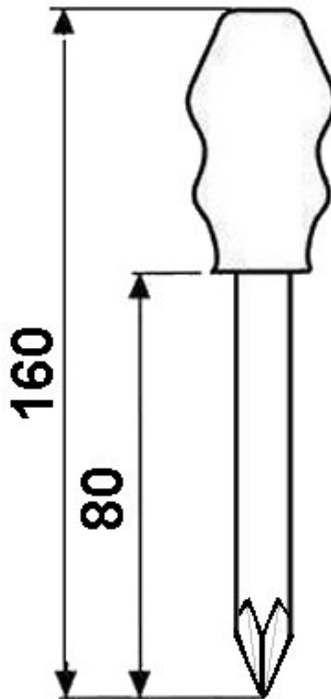
Dimensional drawing
