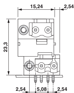
Dimensional drawing
