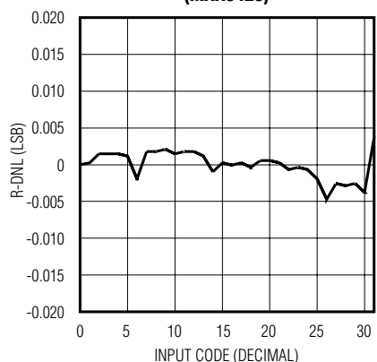
R-DNL ERROR vs. INPUT CODE (MAX5428)
