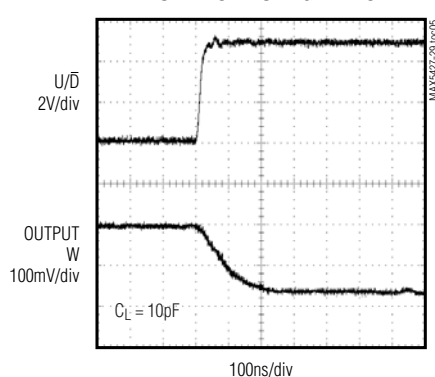
TAP-TO-TAP SWITCHING TRANSIENT
