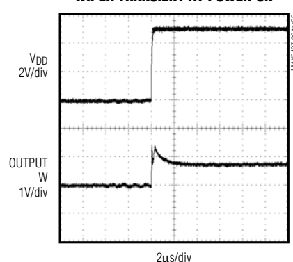
WIPER TRANSIENT AT POWER-ON
