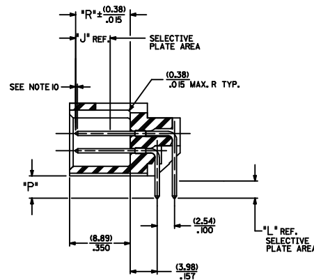
SECTION J-J
