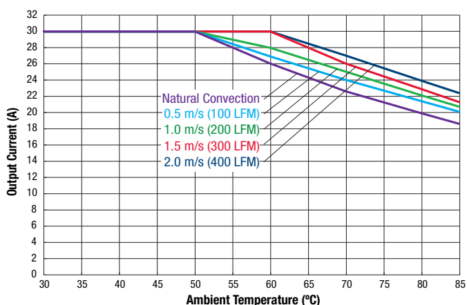
Maximum Current Temperature Derating at Sea Level (Vin = 75V, with baseplate. Airflow Direction Is Longitudinal from Vin to Vout.)
