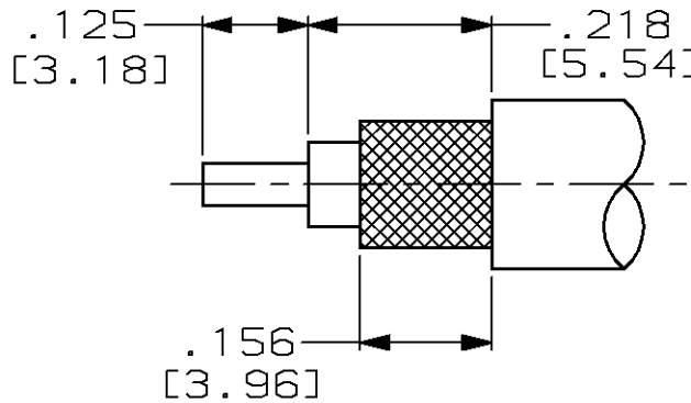
RECOMMENDED STRIP LENGTH SCALE: NTS
