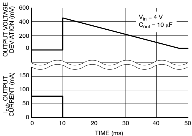
Figure 8. Load Transient Response
