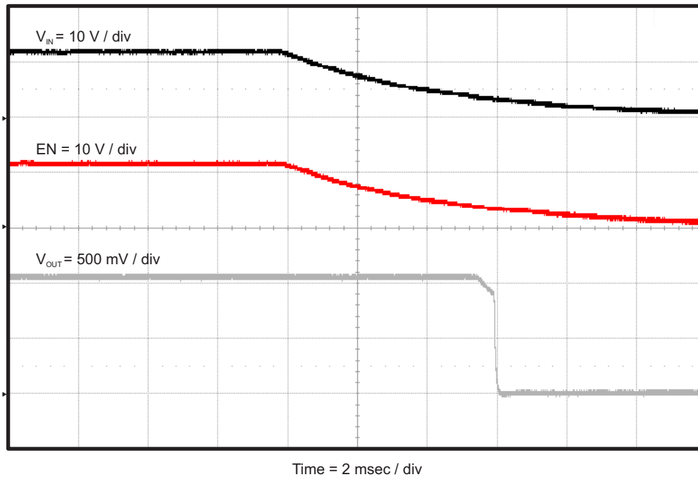
Figure 10. TPS562209EVM-601 Shut-Down Relative to V_{IN}
