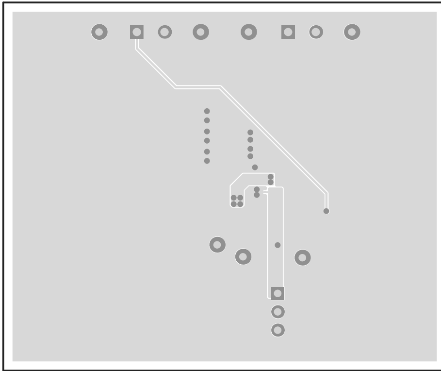
Figure 13. Bottom Layer
