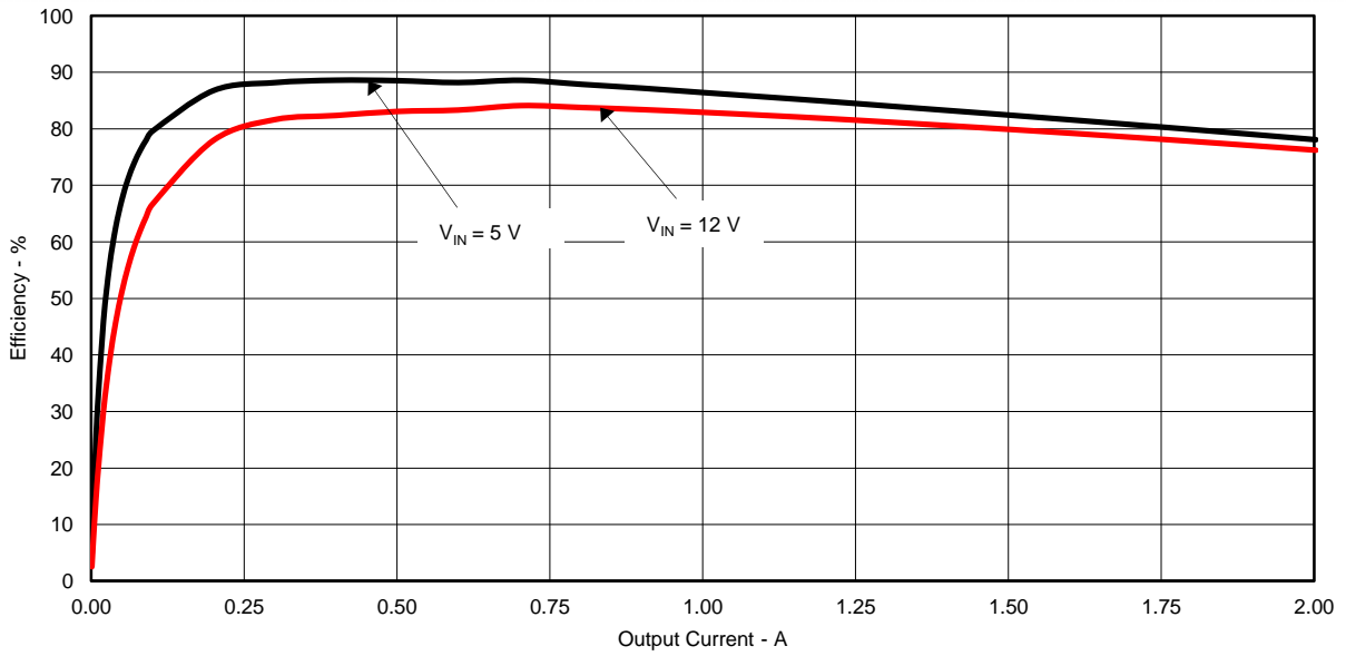
Figure 1. TPS562209EVM-601 Efficiency
