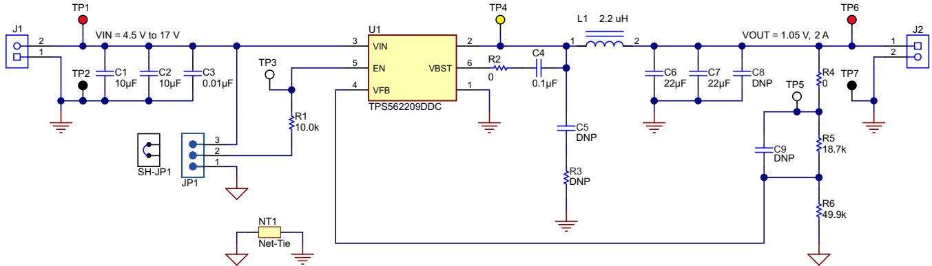
Figure 14. TPS562209EVM-601 Schematic Diagram
