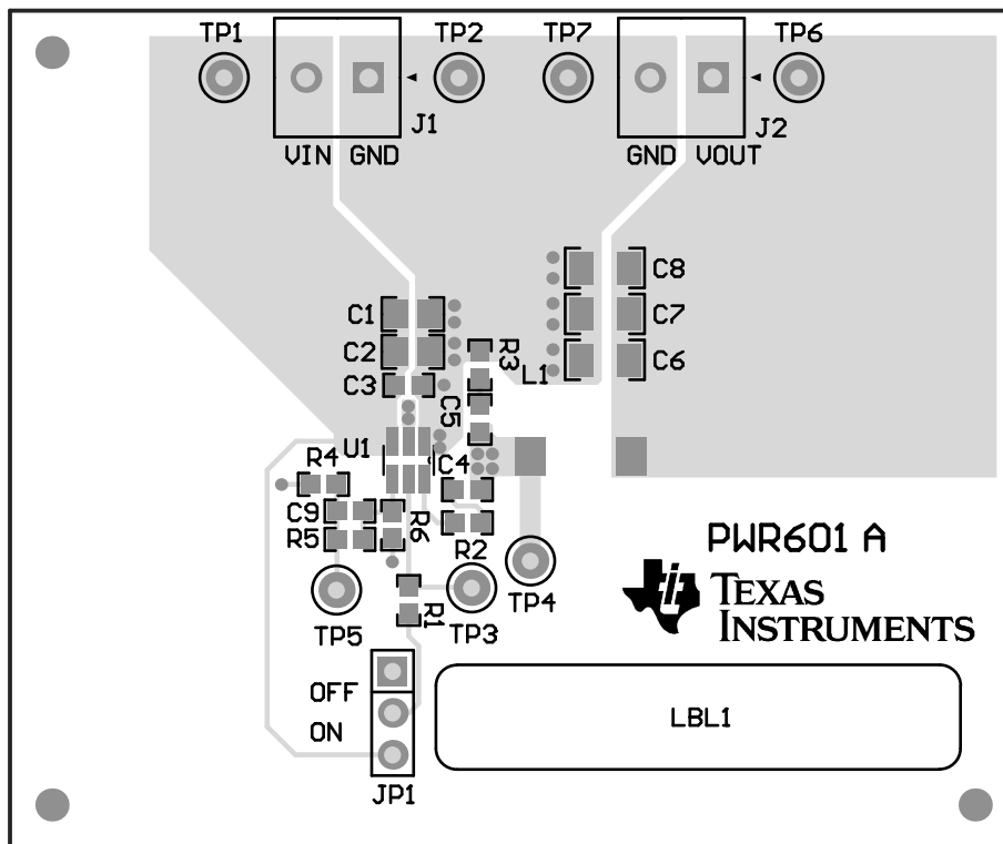
Figure 12. Top Assembly
