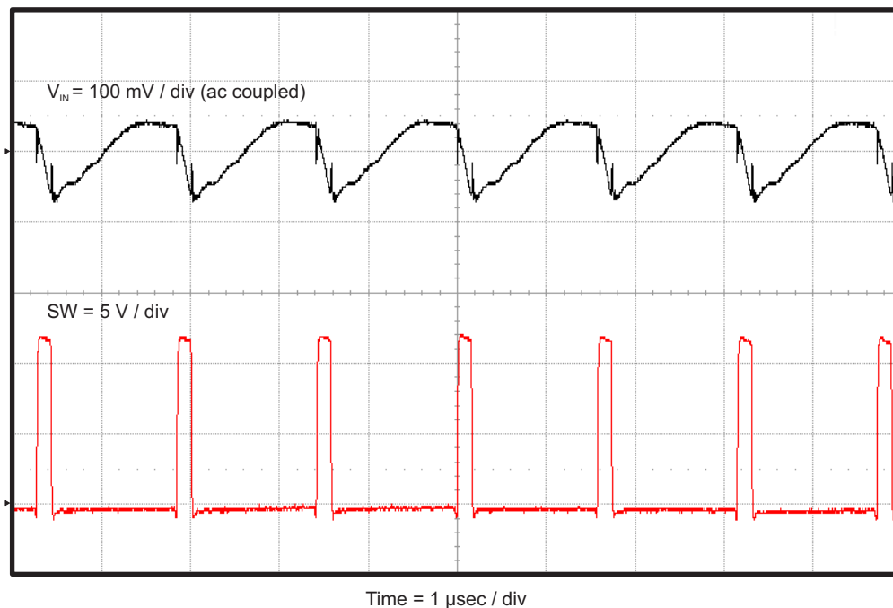
Figure 7. TPS562209EVM-601 Input Voltage Ripple, I_{OUT} = 2\text{ A}
