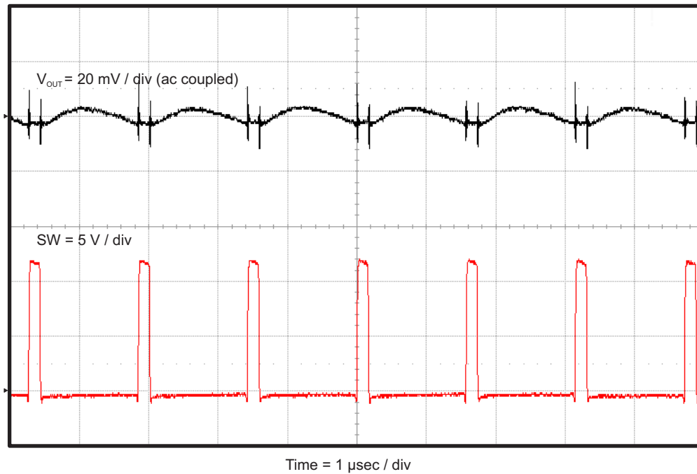
Figure 6. TPS562209EVM-601 Output Voltage Ripple, I_{OUT} = 2\text{ A}
