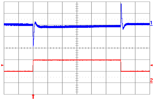
Fig. 10: Output voltage response to load current step-change (20 A – -20 A) at V_{in} = 48\text{ V} . Top trace: output voltage (100 mV/div.). Bottom trace: load current (10 A/div.). Current slew rate: 5 A/ \mu\text{s} . C_o = 470\ \mu\text{F} POS + 1 \mu\text{F} ceramic. Time scale: 0.2 ms/div.
