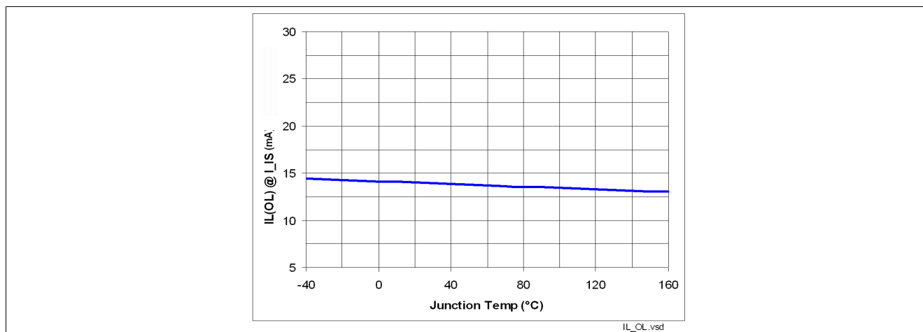
Figure 46 Open Load Detection ON State Threshold I_{L(OL)} = f(T_J; V_S)
