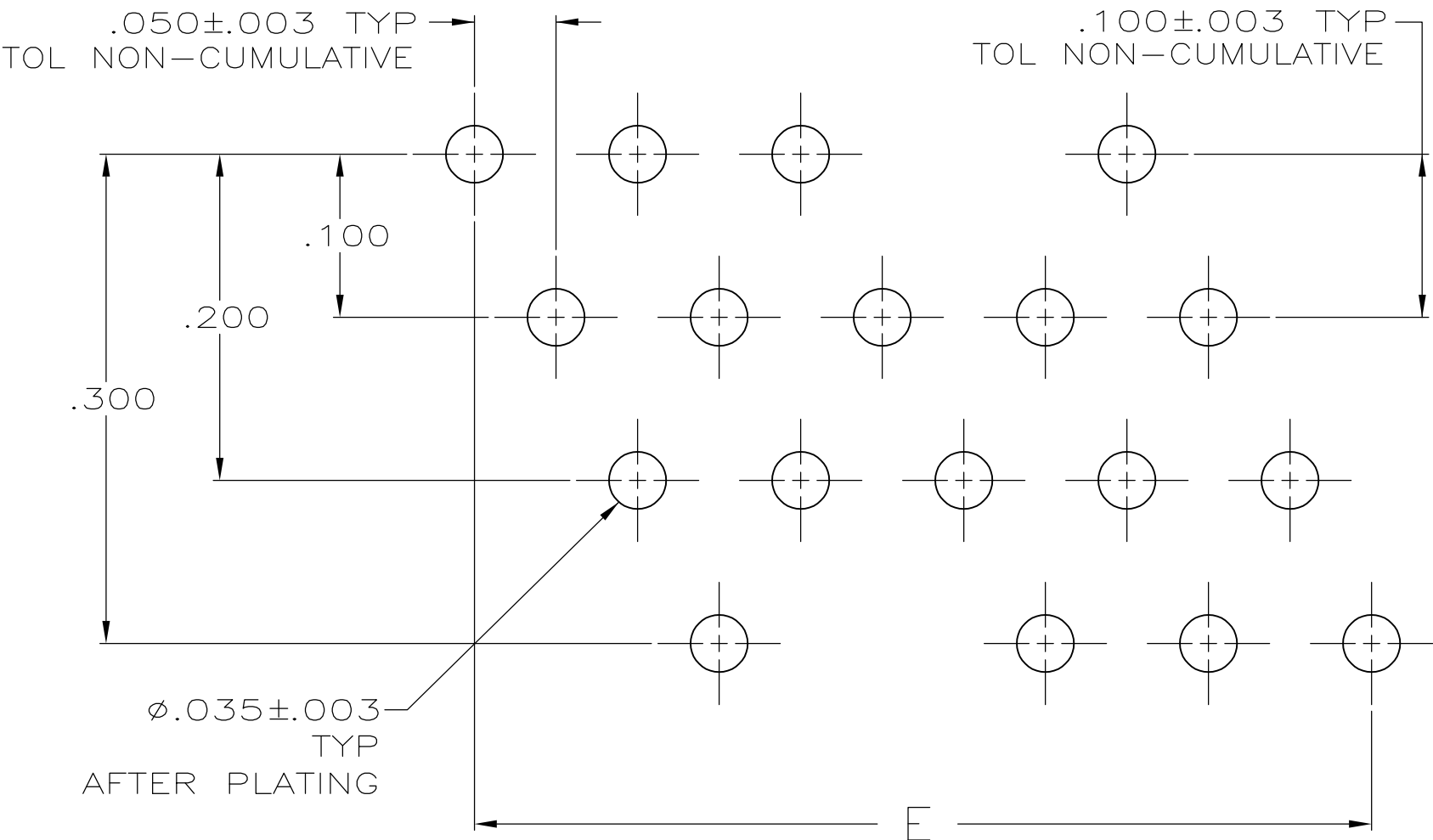
RECOMMENDED HOLE LAYOUT
