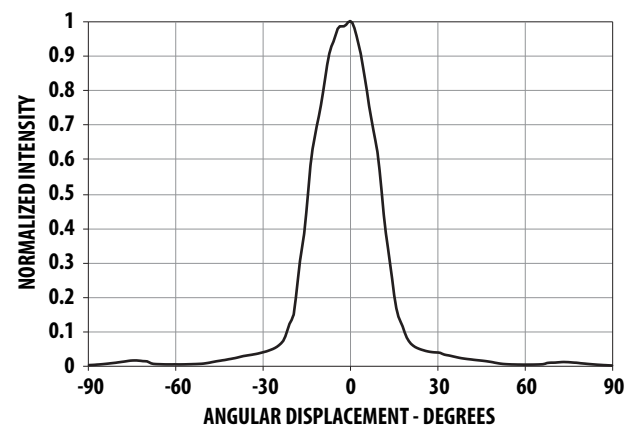
Figure 8: Representative Radiation Pattern for 23° Viewing Angle Lamp
