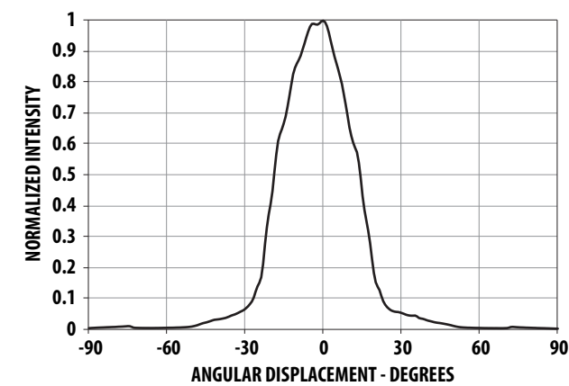
Figure 9: Representative Radiation Pattern for 30° Viewing Angle Lamp
